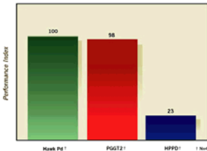
14M Life Comparison (28T PowerGrip GT2, 1750 RPM, Rated Load)
