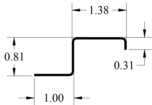
13/16" Z-Section
