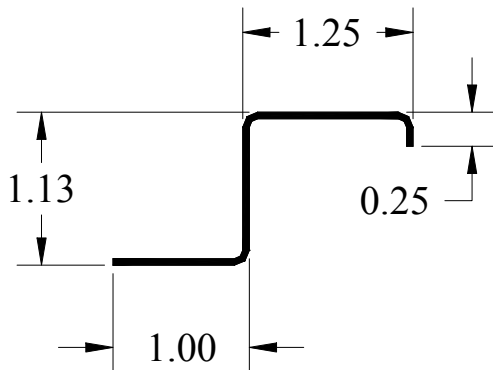
1-1/8" Z-Section
