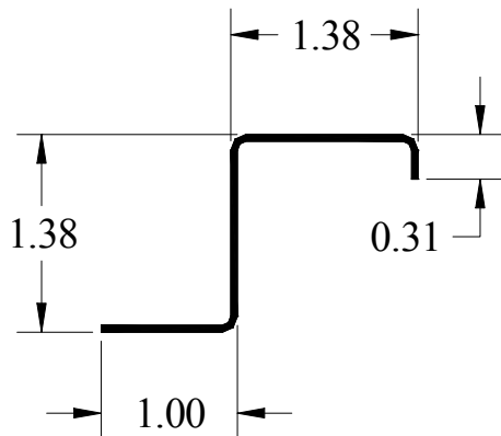
1-3/8" Z-Section
