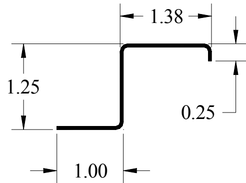
1-1/4" Z-Section
