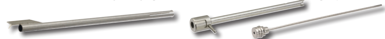
Medical implement for carpal tunnel surgery is an assembly of notched and flared tubing laser welded to a forked scalpel. Two examples of laser welded assemblies are shown above.
