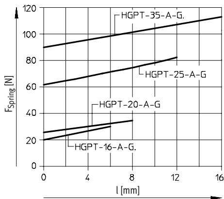
Piston Ø 16 ... 35
