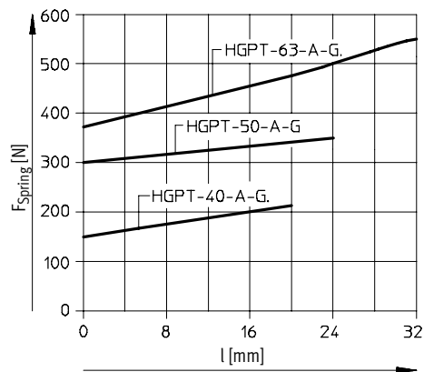
Piston Ø 40 ... 63
