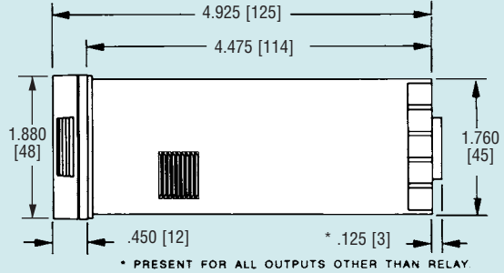
PANEL CUTOUT FOR ALL MODELS 1.772" X 1.772" [45 mm X 45 mm] ALLOW FOR 0.5" [13 mm] CLEARANCE AT THE REAR OF INSTRUMENT.
