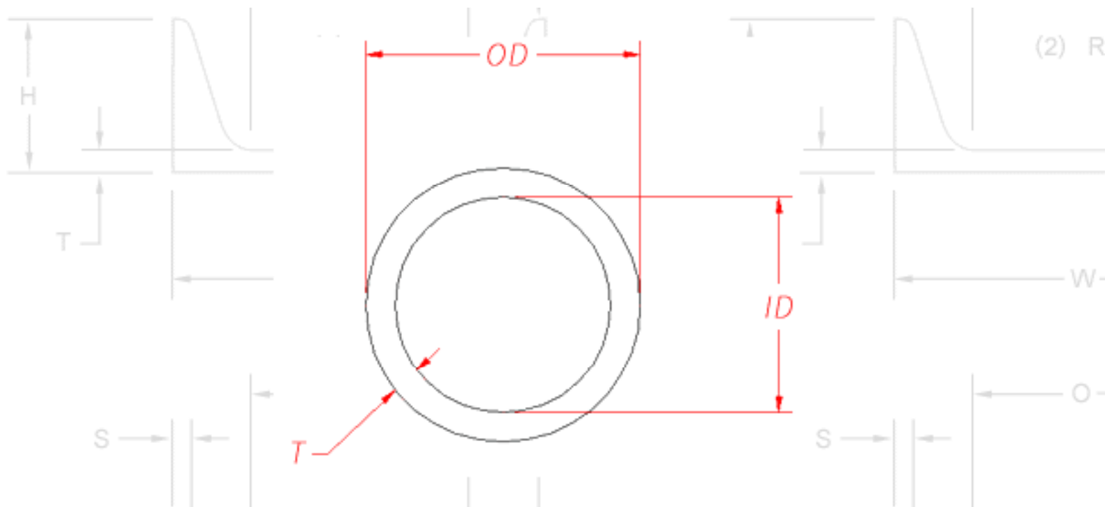
Schedule 40 - Pipe
