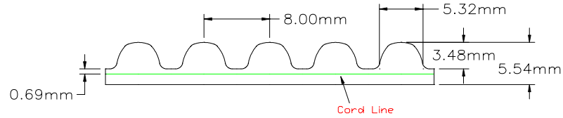
Dimensions in millimeters
