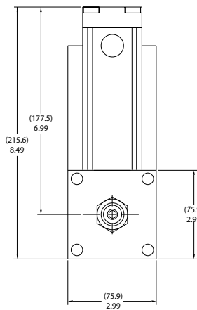
C180H, H1, H2 Side View
