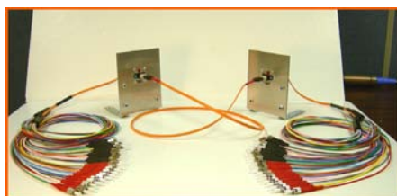
Panel mount MTP Conversion Fixtures that replace M28876 Connectors
