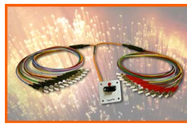
24 Fiber MTP to ST Fan Out with MTP Conversion Fixture.
