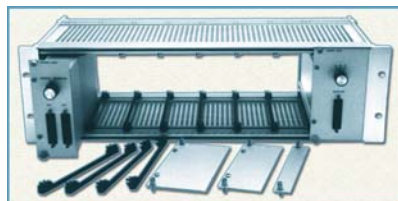
Model 9025 Rack Chassis illustrated with other switch modules and optional filler panels.
